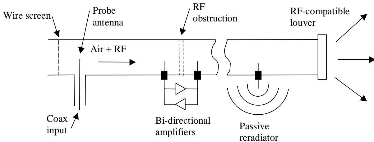
Figure 1. Major components of an HVAC RF distribution system.
